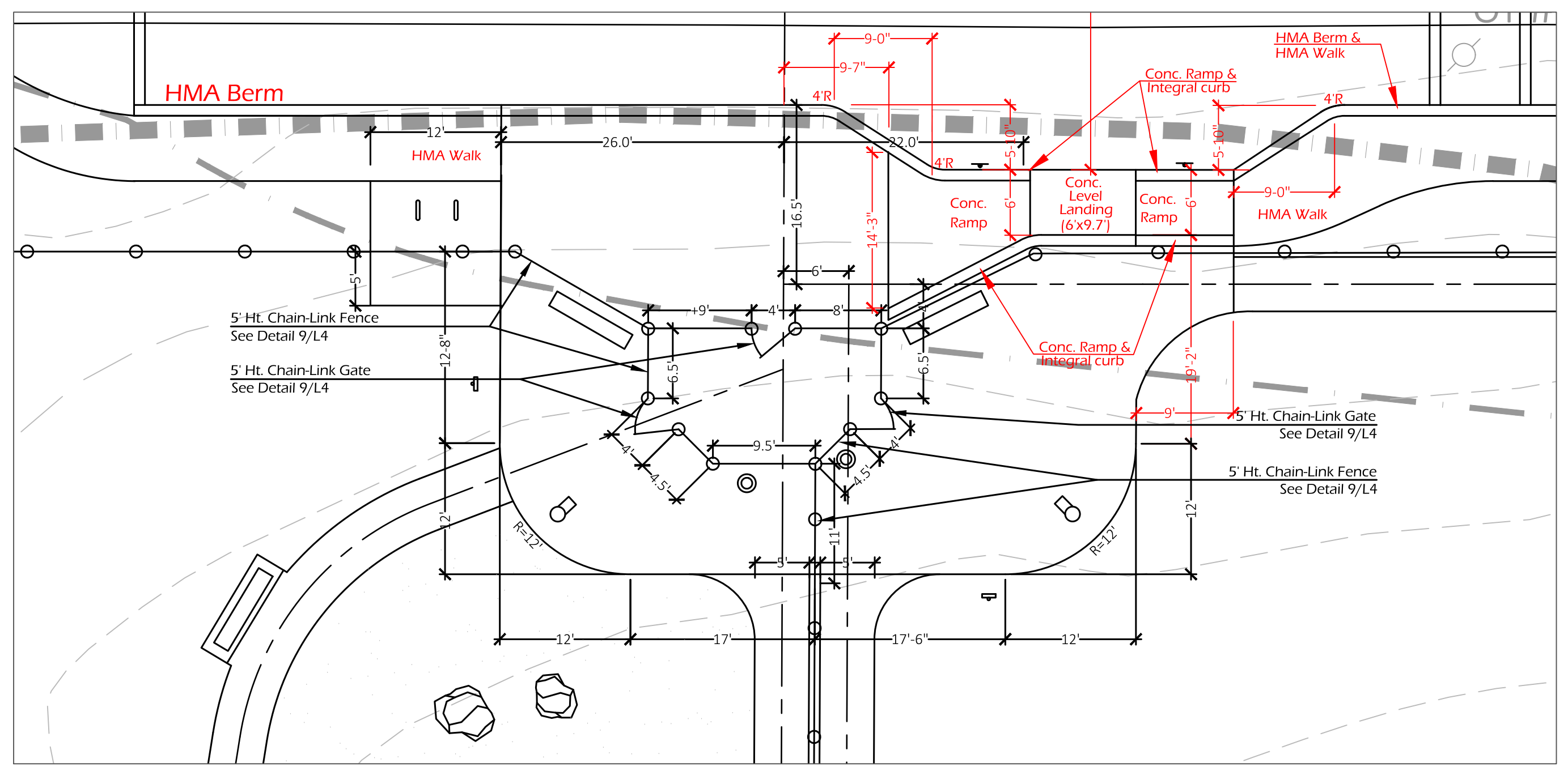
Inset-Entrance Layout
